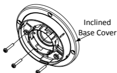
Figure 2-7 Install Turret Camera's Mounting Base
