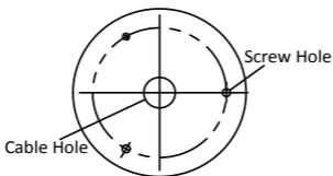
Figure 2-2 Drill Template
