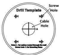
Figure 2-12 Drill Template of the Junction Box
