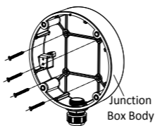
Figure 2-14 Secure the Junction Box's Body on Wall / Ceiling
