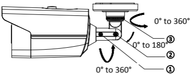
Figure 2-10 3-Axis Adjustment
