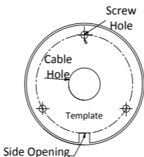
Figure 2-8 Drill Template
