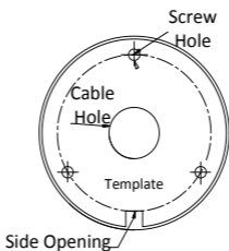
Figure 2-1 Drill Template
