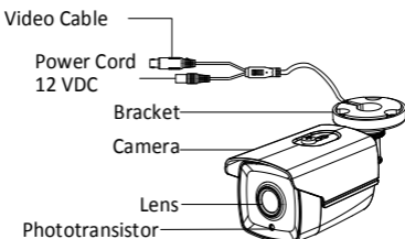
Figure 1-2 Overview of Type II Camera
