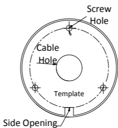
Figure 2-4 Drill Template of Junction Box
